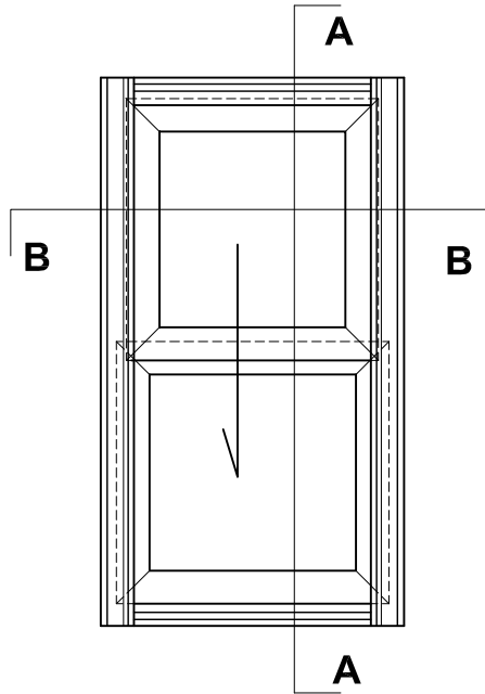
DOUBLE HUNG TILT Exterior View
