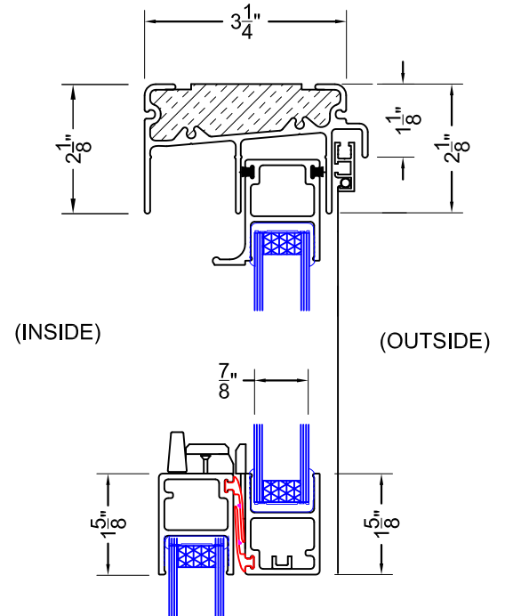
HEAD DETAIL
