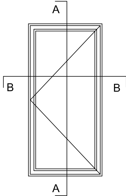
CASEMENT WINDOW EXTERIOR VIEW CLOSED BACK FRAME
